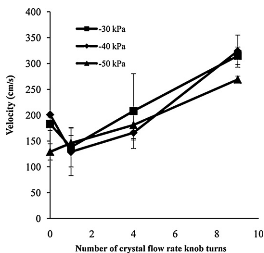
Fig. A3. Average crystal particle velocity shown as a function of the number of turns of the crystal flow rate knob at different suction pressures. Data represent the average of 20 particle measurements \pm standard deviation.
