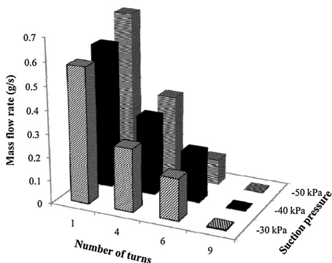
Fig. A2. Mass flow rate is shown as a function of suction pressure and number of turns of the crystal flow rate knob applied in the static mode. Data represent the average of three replicate measurements. Error bars are not shown to simplify the presentation. The magnitude of the error bars in these data is similar to those shown in Fig. A1.
