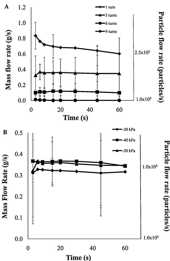
Fig. A1. Crystal mass flow rate and particle flow rate shown as a function of time at different crystal knob turns and suction pressures. (A) Mass and particle flow rates at 1, 3, 6, and 9 knob turns at a suction pressure of -50 kPa in the static mode. (B) Mass and particle flow rate at suction pressures of -30 , -40 , and -50 kPa at a crystal flow rate at 3 turns in the static mode. Data represent the average of three replicate measurements \pm standard deviation.
